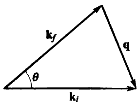
Figure 13.7 The incident wave vector k_i , the scattered wave vector k_f , and the vector q = k_i - k_f .
