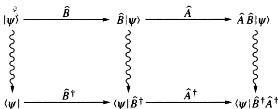
Figure 2.8 The adjoint of the product of operators is determined by the correspondence between bras and kets.
