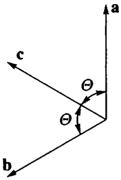
Figure 5.7 An orientation of the axes \mathbf{a} , \mathbf{b} , and \mathbf{c} where \mathbf{c} bisects the angle between \mathbf{a} and \mathbf{b} .
