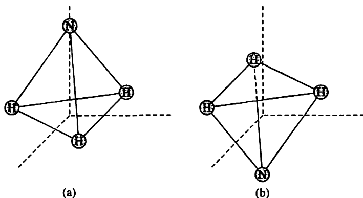
Figure 11.6 The action of the parity operator on state |I\rangle of the \text{NH}_3 molecule, with the N atom above the plane formed by the three H atoms, as shown in (a), produces state |II\rangle , with the N atom below the plane, as shown in (b).
