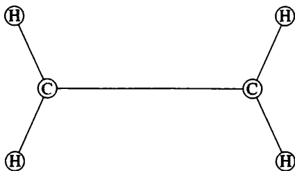
Figure 7.4 The planar structure of the ethylene molecule, C_2H_4 .
