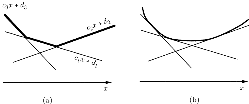
Figure 1.2: (a) A piecewise linear convex function of a single variable. (b) An approximation of a convex function by a piecewise linear convex function.
