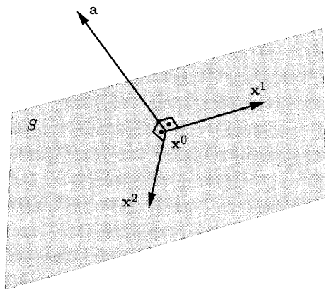
Figure 1.7: Consider a set S in \mathfrak{R}^3 defined by a single equality constraint \mathbf{a}'\mathbf{x} = b . Let \mathbf{x}^0 be an element of S . The vector \mathbf{a} is perpendicular to S . If \mathbf{x}^1 and \mathbf{x}^2 are linearly independent vectors that are orthogonal to \mathbf{a} , then every \mathbf{x} \in S is of the form \mathbf{x} = \mathbf{x}^0 + \lambda_1 \mathbf{x}^1 + \lambda_2 \mathbf{x}^2 . In particular, S is a two-dimensional affine subspace.
