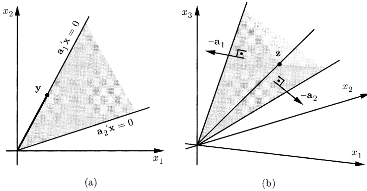
Figure 4.12: Extreme rays of polyhedral cones. (a) The vector y is an extreme ray because n = 2 and the constraint \mathbf{a}'_1\mathbf{x} = 0 is active at y . (b) A polyhedral cone defined by three linearly independent constraints of the form \mathbf{a}'_i\mathbf{x} \geq 0 . The vector \mathbf{z} is an extreme ray because n = 3 and the two linearly independent constraints \mathbf{a}'_1\mathbf{x} \geq 0 and \mathbf{a}'_2\mathbf{x} \geq 0 are active at \mathbf{z} .
