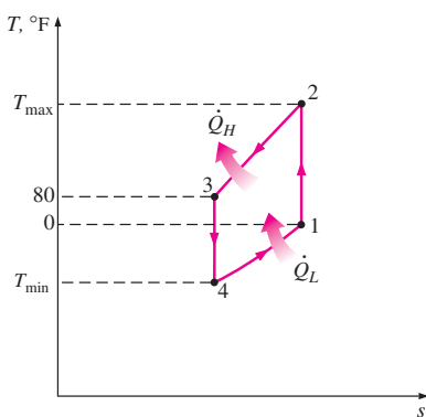
FIGURE 11-20 T - s diagram of the ideal-gas refrigeration cycle described in Example 11-5.
