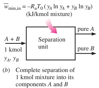
FIGURE 13–23 The minimum work required to separate a two-component mixture for the two limiting cases.
