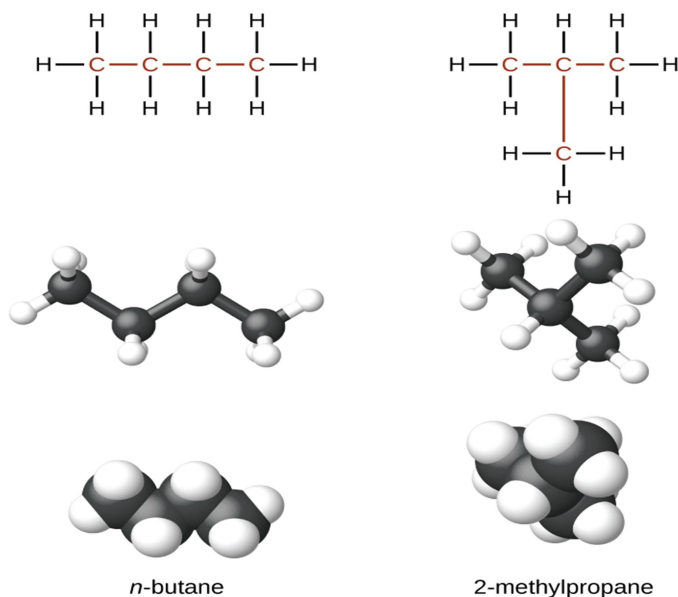
Figure 8.3:- Structure for n -butane and 2-methylpropane
