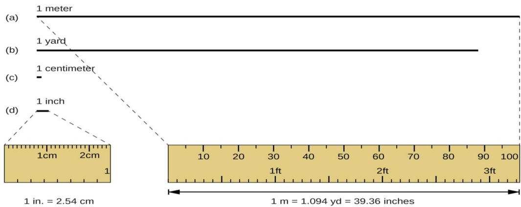
Figure 1.12: The relative lengths of 1 m, 1 yd, 1 cm, and 1 in. are shown (not actual size), as well as comparisons of 2.54 cm and 1 in., and of 1 m and 1.094 yd.
