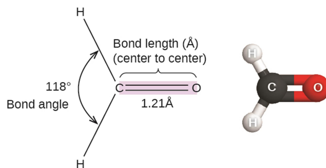
Figure 6.6: Bond distances (lengths) and angles are shown for the formaldehyde molecule, H 2 CO.
