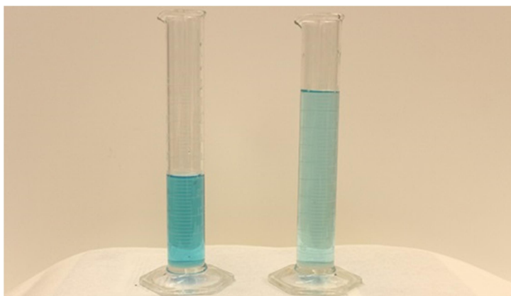
Figure 3.9: This figure shows two graduated cylinders side-by-side. Both solutions contain the same mass of copper nitrate. The solution on the right is more dilute because the copper nitrate is dissolved in more solvent. The first has about half as much blue liquid as the second. The blue liquid is darker in the first cylinder than in the second.
