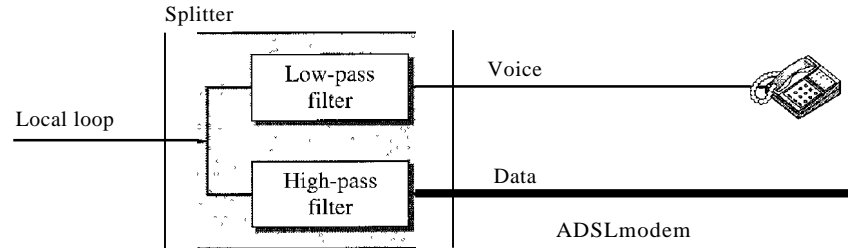
Figure 9.12 ADSL modem
