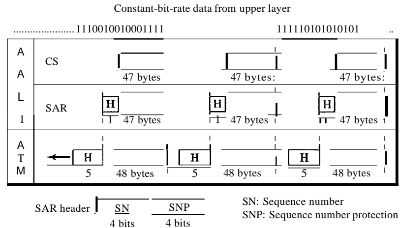
Figure 18.20 AAL1
